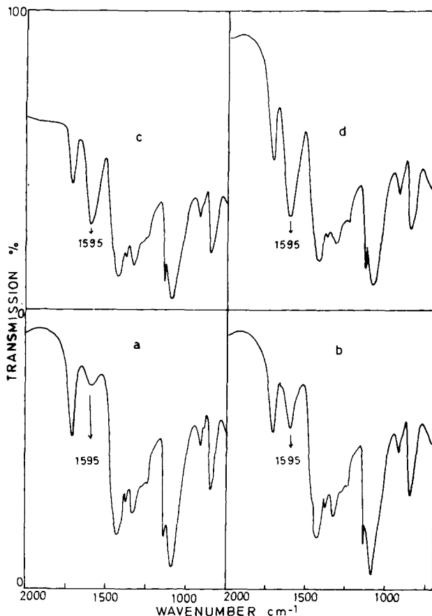
Fig. 4. Partial infrared spectra of \gamma -irradiated ZnCl 2 -treated PVA (KOH/ZnCl 2 = 1): (a) treated with 5 wt %; (b) treated with 10 wt %; (c) treated with 20 wt %; (d) treated with 30 wt %.
