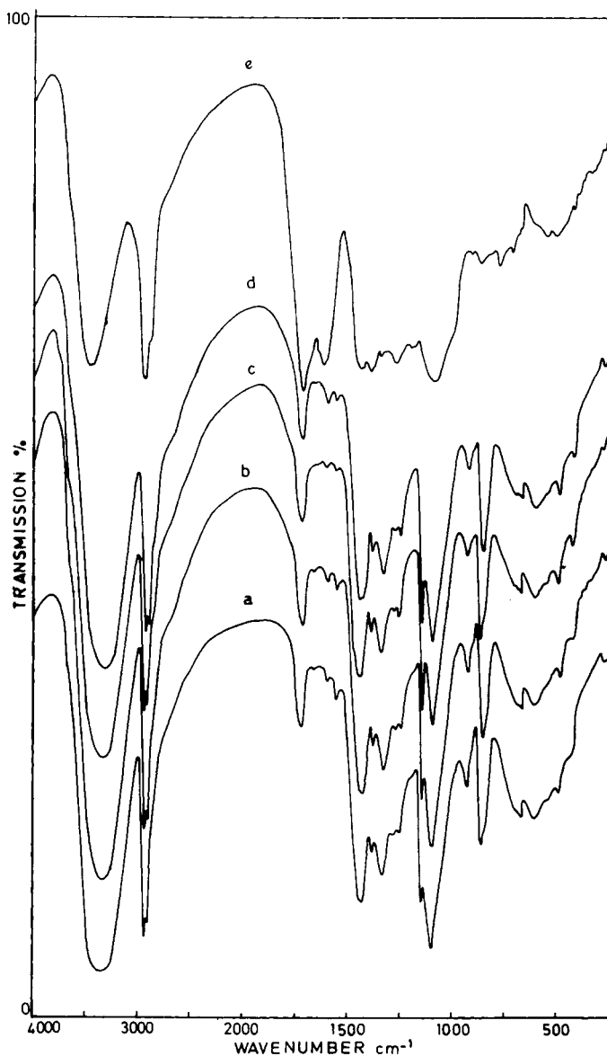
Fig. 7. Infrared spectra of treated samples 5 wt % and \text{KOH}/\text{ZnCl}_2 = 2 heated in air at: (a) room temperature; (b) 60^\circ\text{C} ; (c) 90^\circ\text{C} ; (d) 120^\circ\text{C} ; (e) 150^\circ\text{C} .
