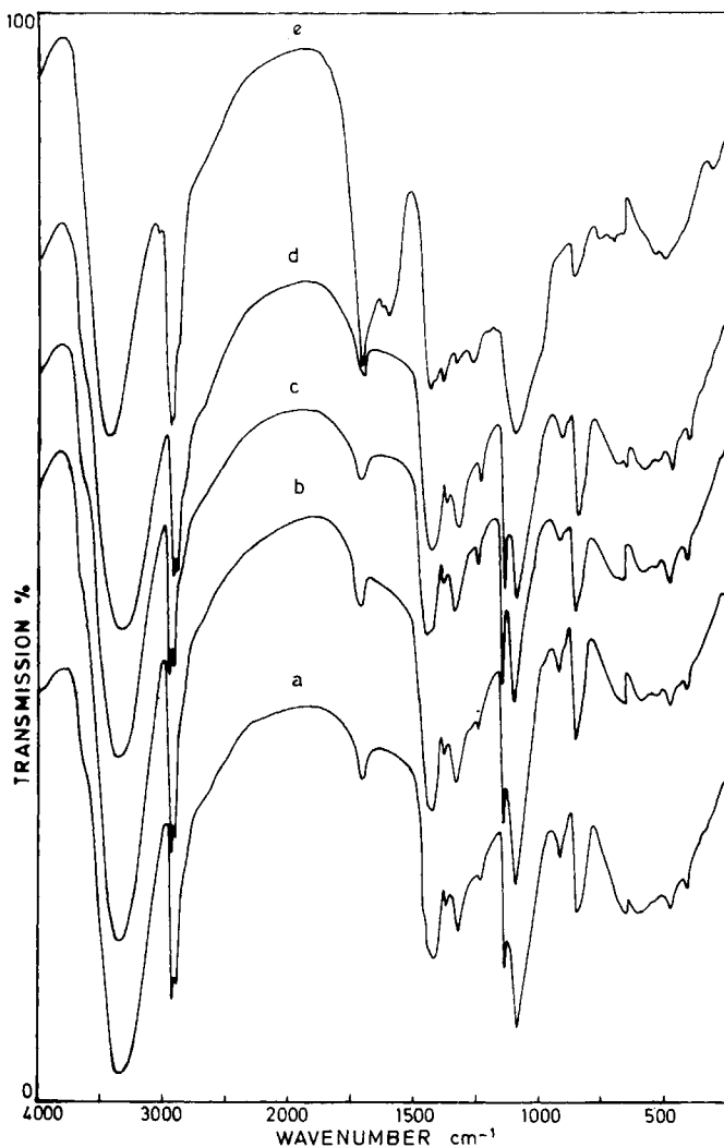
Fig. 8. Infrared spectra of \text{ZnCl}_2 -treated sample 10 wt % and \text{KOH}/\text{ZnCl}_2 = 2 heated in air at: (a) room temperature; (b) 60^\circ\text{C} ; (c) 90^\circ\text{C} ; (d) 120^\circ\text{C} ; (e) 150^\circ\text{C} .
