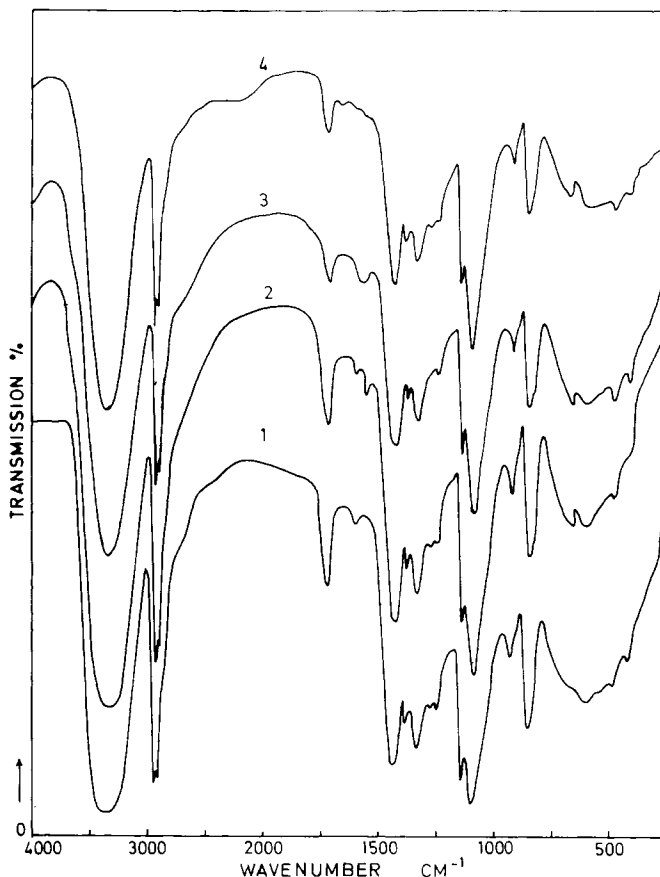
Fig. 2. Infrared spectra of ZnCl 2 -treated PVA: (1) untreated PVA; (2) treated with 5% ZnCl 2 and KOH/ZnCl 2 = 2; (3) treated with 10% ZnCl 2 and KOH/ZnCl 2 = 2; (4) treated with 20% ZnCl 2 and KOH/ZnCl 2 = 2.
