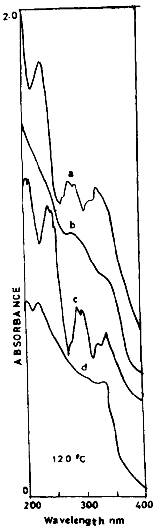
Fig. 11. The ultraviolet spectra of samples heated at 120°C: (a) treated with 20 wt % \text{KOH}/\text{ZnCl}_2 = 1 ; (b) treated with 20 wt % \text{KOH}/\text{ZnCl}_2 = 2 ; (c) treated with 30 wt % \text{KOH}/\text{ZnCl}_2 = 1 ; (d) treated with 30 wt % \text{KOH}/\text{ZnCl}_2 = 2 .
