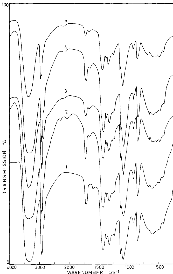
Fig. 1. Infrared spectra of \text{FeCl}_3 -treated PVA: (1) untreated PVA; (2) treated with 10% \text{FeCl}_3 and \text{KOH}/\text{FeCl}_3 = 1 ; (3) treated with 10% \text{FeCl}_3 and \text{KOH}/\text{FeCl}_3 = 2 ; (4) treated with 20% \text{FeCl}_3 and \text{KOH}/\text{FeCl}_3 = 1 ; (5) treated with 20% \text{FeCl}_3 and \text{KOH}/\text{FeCl}_3 = 2 .
